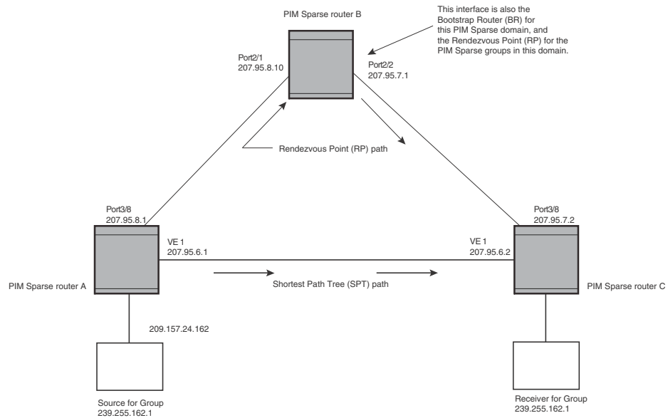
FIGURE 92 Example PIM Sparse domain
