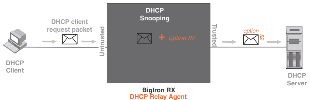
FIGURE 131 DHCP option 82 is added to the packet
