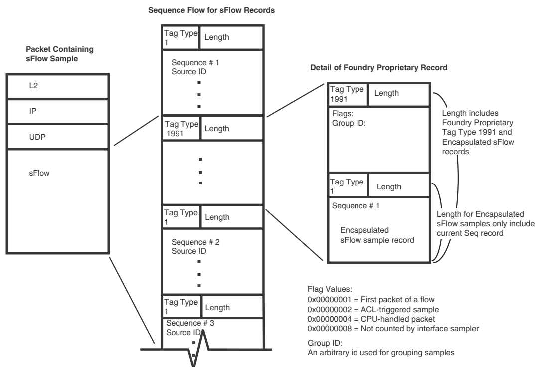
FIGURE 133 sFlow packet format
