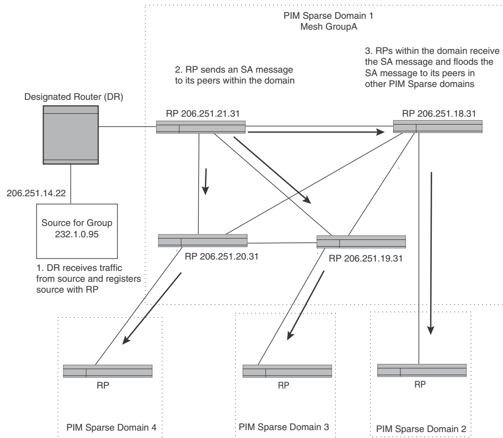
FIGURE 94 Example of MSDP mesh group
