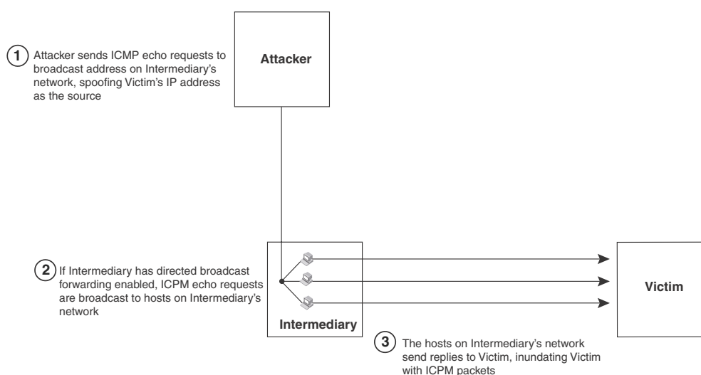
FIGURE 127 How a Smurf attack floods a victim with ICMP replies
