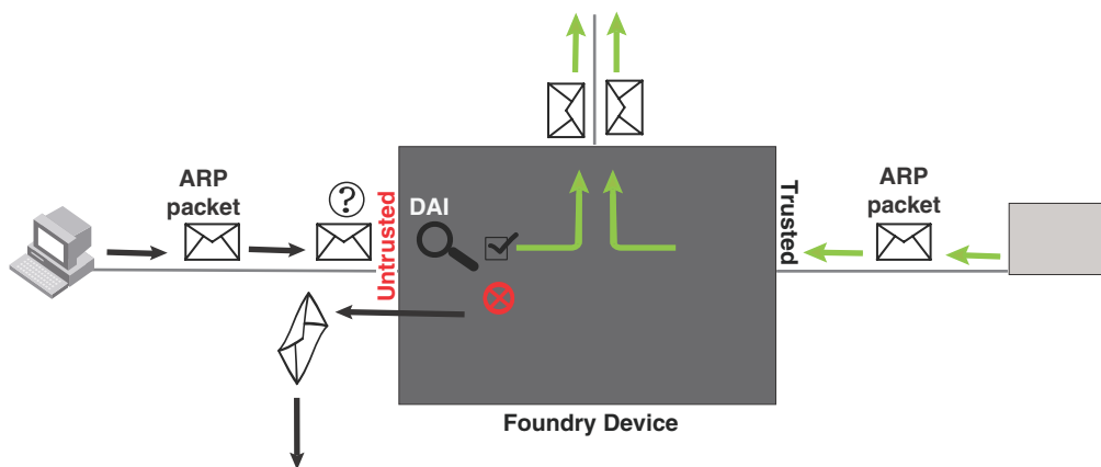
FIGURE 128 Dynamic ARP Inspection at work
