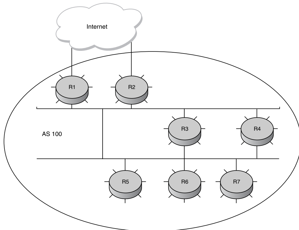
FIGURE 113 Sample Null0 routing application
