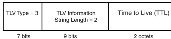
FIGURE 19 TTL TLV packet format
