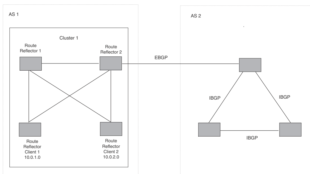
FIGURE 115 Example route reflector configuration
